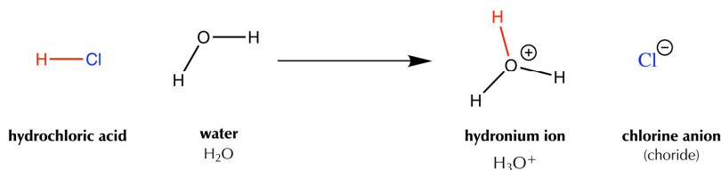
Figure 2. Strong Acid Solvation
