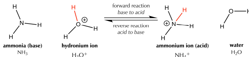
Figure 3. Ammonia Equilibrium
