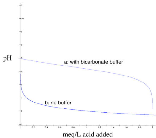
Figure 7. Buffer slows pH drop upon acid addition
