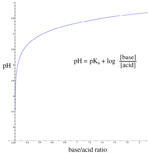
Figure 6. Henderson-Hasselbalch Equation
