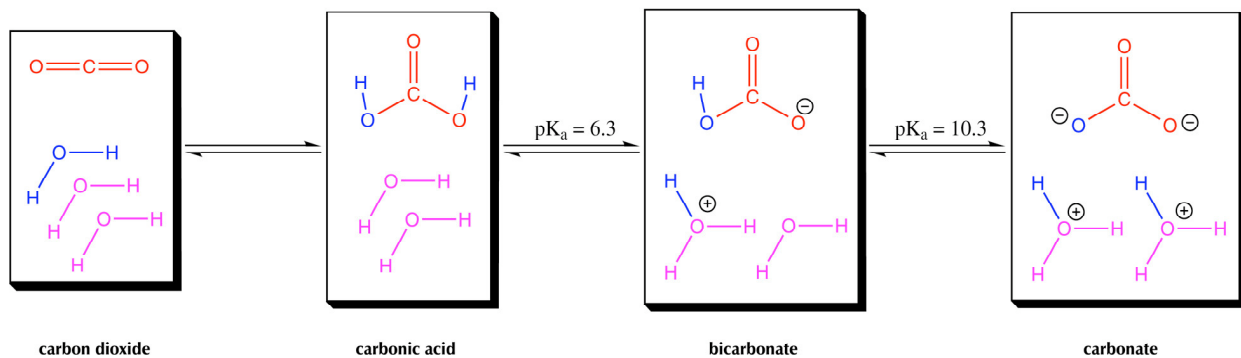
Figure 9. The Carbonate Buffer Equilibrium
